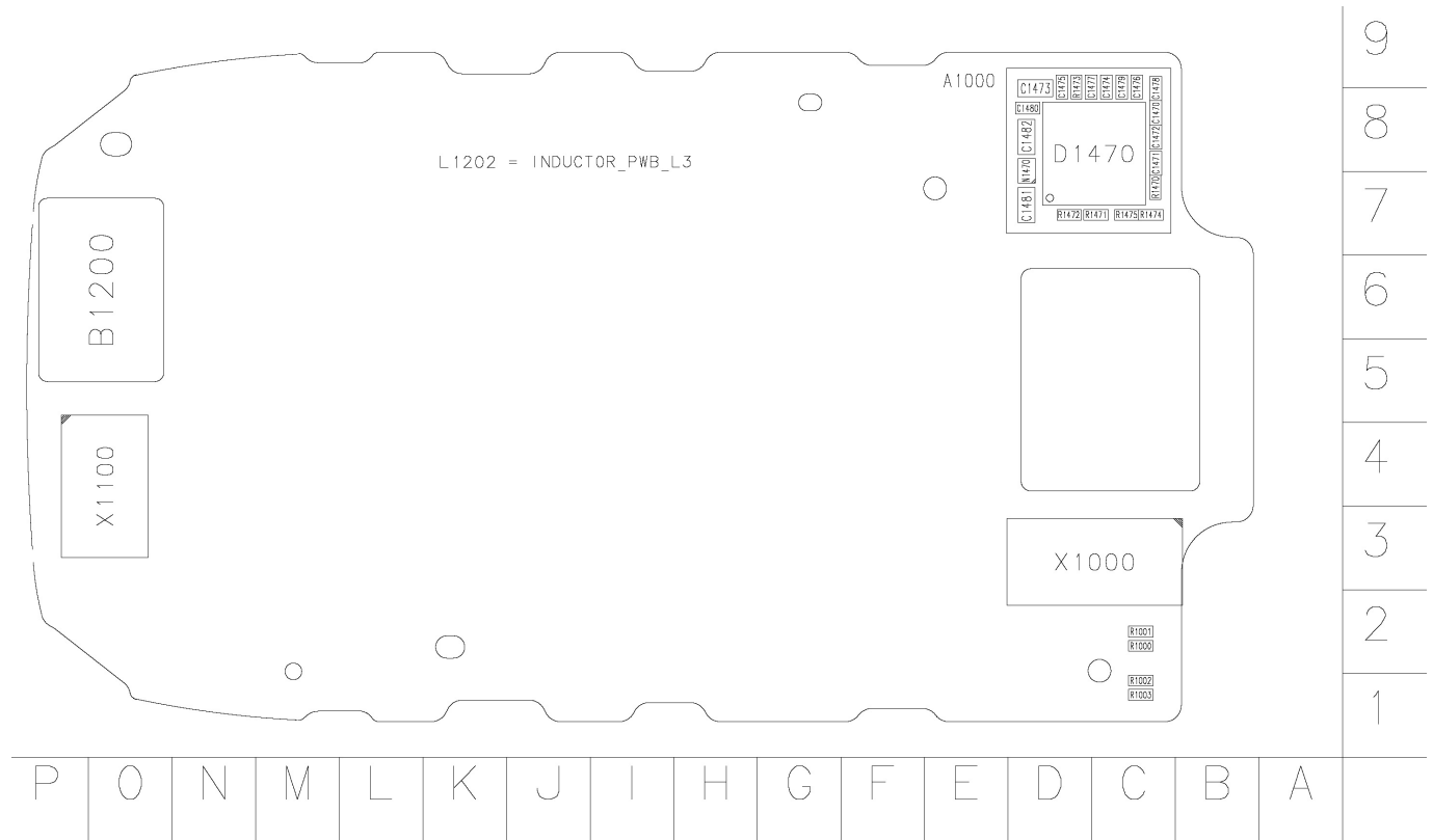
Figure 4 Component layout - bottom (1Iha_50a)
